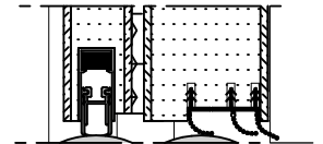
Lip seal
